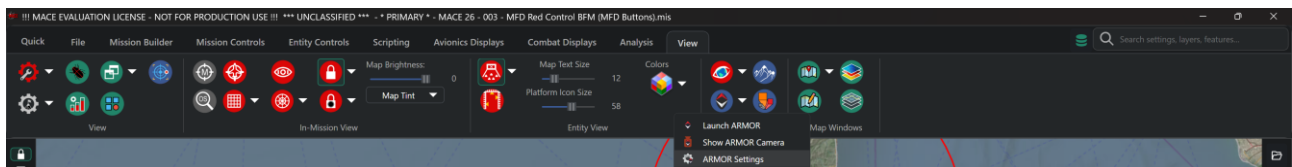
Figure 6: MACE-ARMOR Plugin
